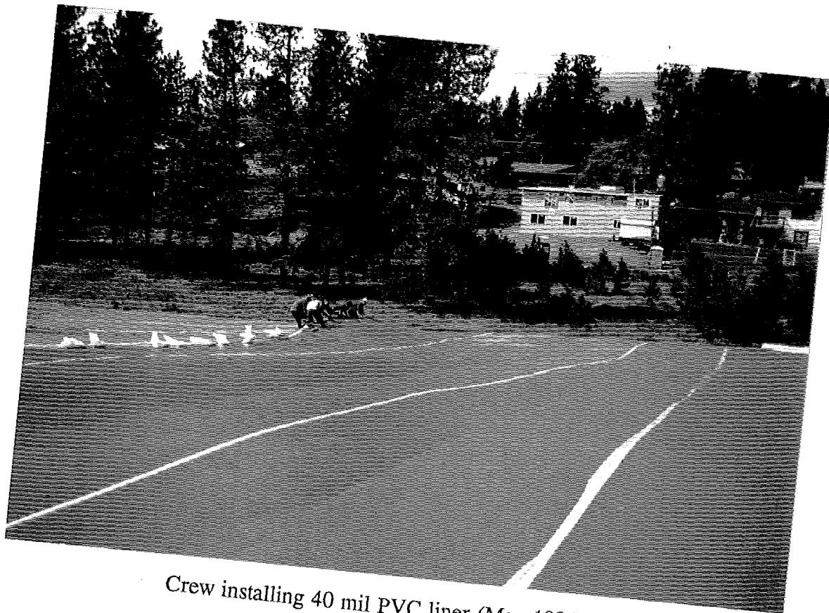
Dust control during cap installation was an important part of construction activities (May 1994).
